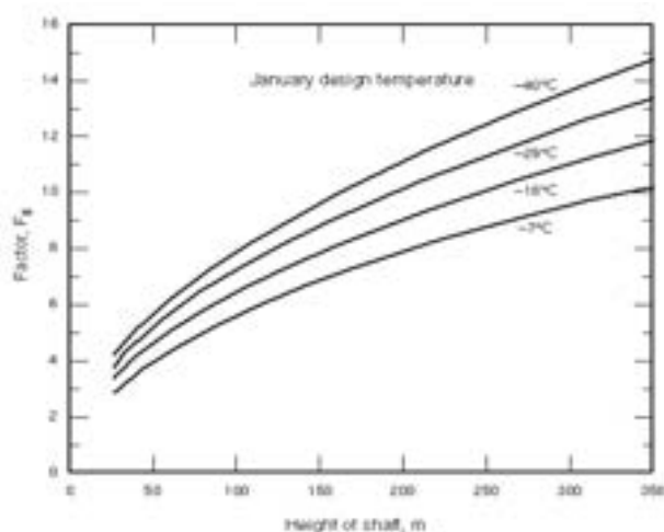
Graph 4 Factor for air supply to an elevator shaft
