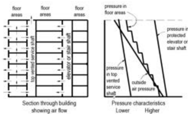
Figure 23 Pressure characteristics in a Measure F building
