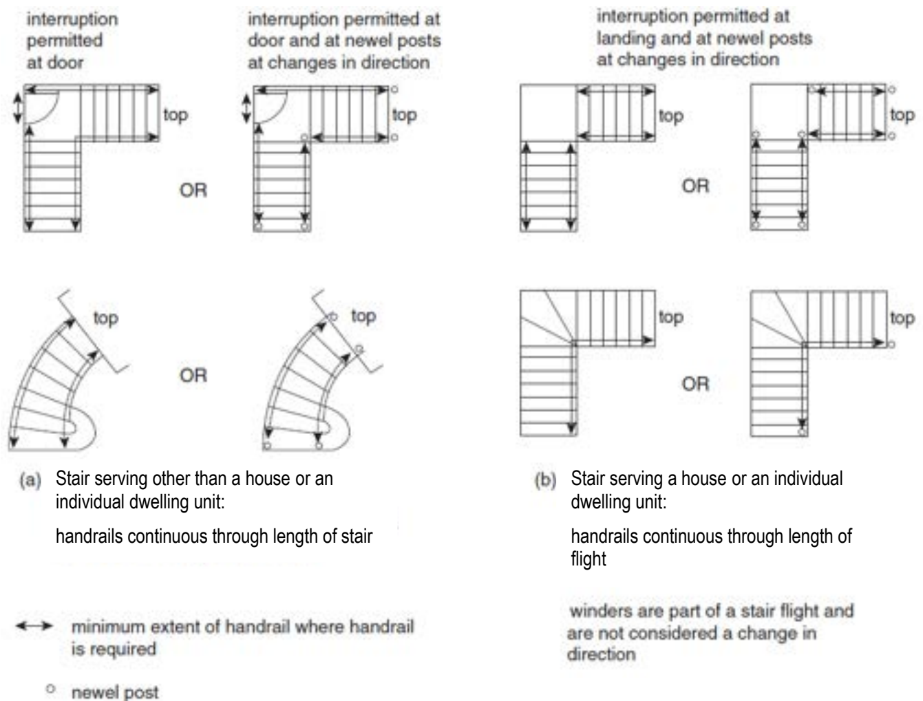
Figure A-9.8.7.2. Continuity of Handrails at the Top and Bottom of Stairs and Flights of Stairs
