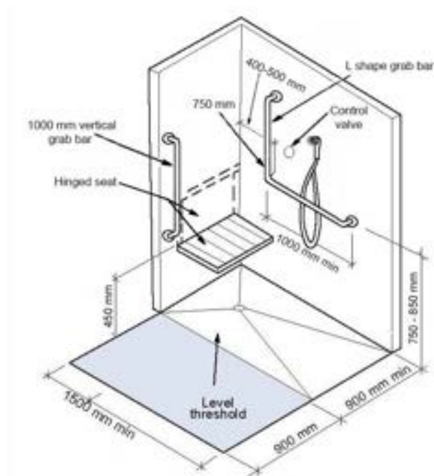
Figure A-3.8.3.13.(2)(e), (f) and (g) Accessible Shower
