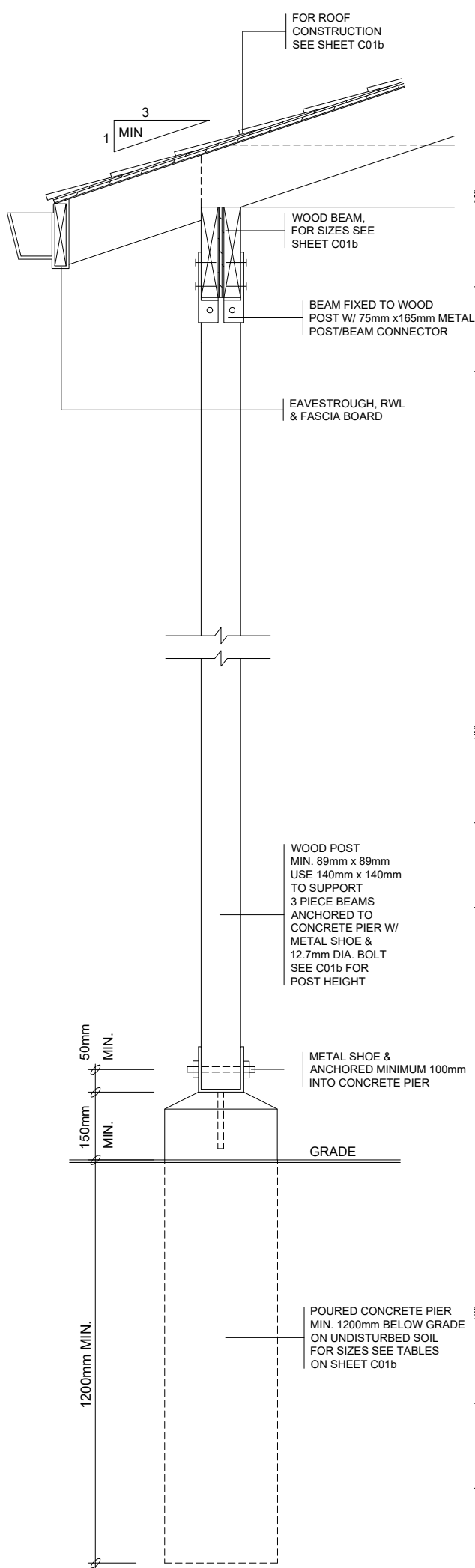
4 SUPPORT DETAIL
