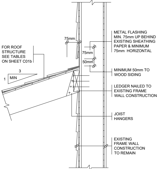
1 FRAME WALL
