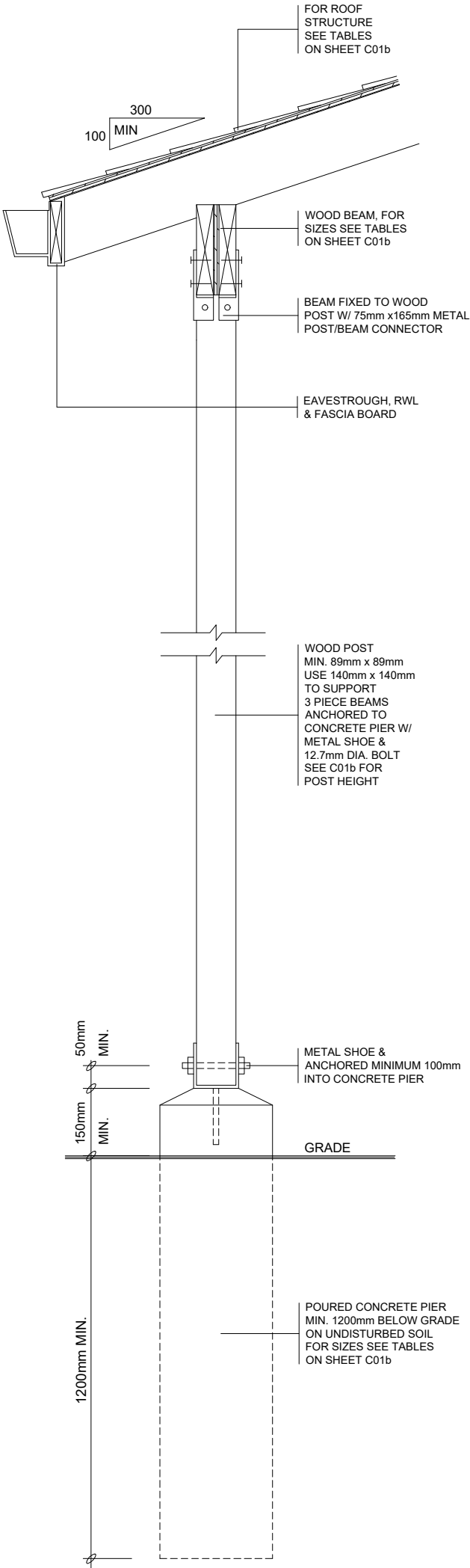
4 SUPPORT DETAIL
