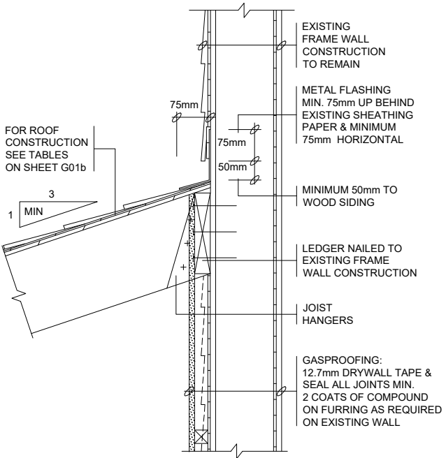
1 FRAME WALL
