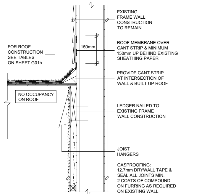
1 FRAME WALL
