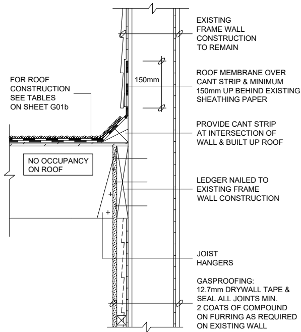
1 FRAME WALL
