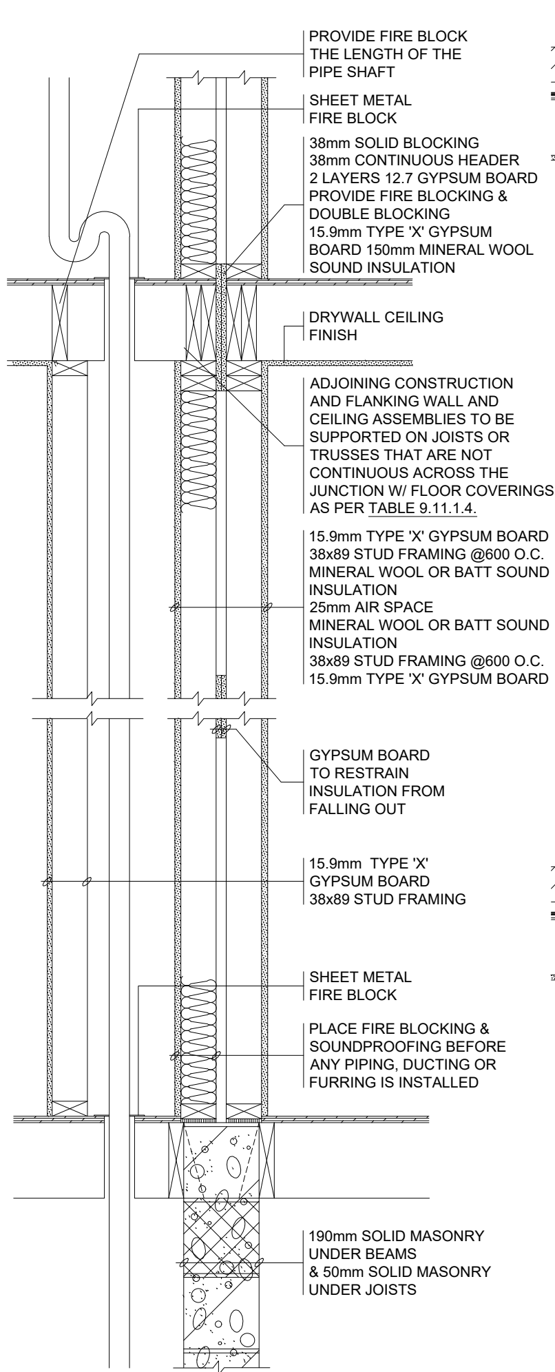
VERTICAL SECTION
