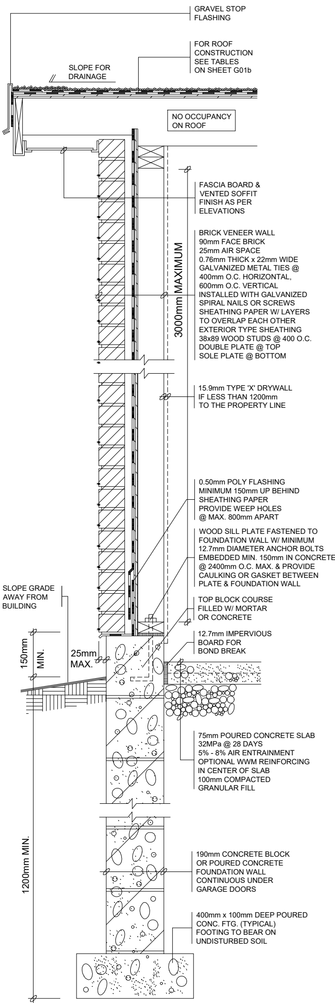
4 WALL SECTION
