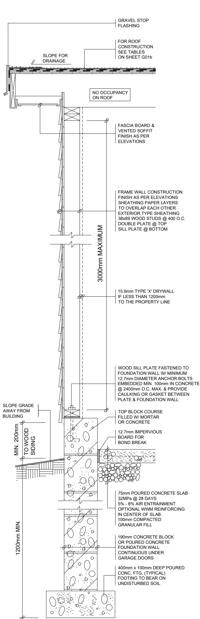
4 WALL SECTION
