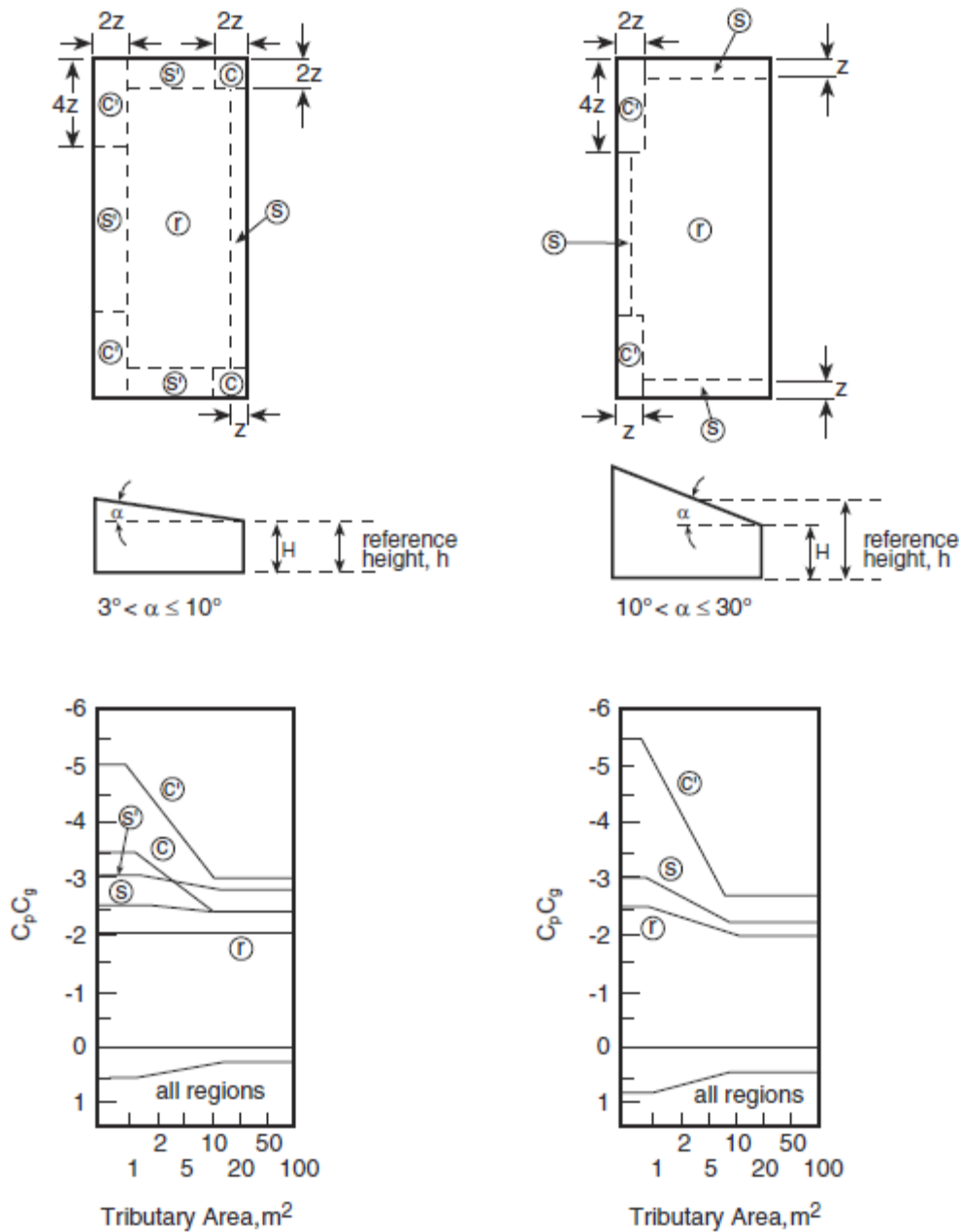
Figure 4.1.7.6.G. External Peak Values of C_p C_q on Monoslope Roofs for the Design of Structural Components and Cladding (1)(2)(3)(4) Forming Part of Sentence 4.1.7.6.(8)
