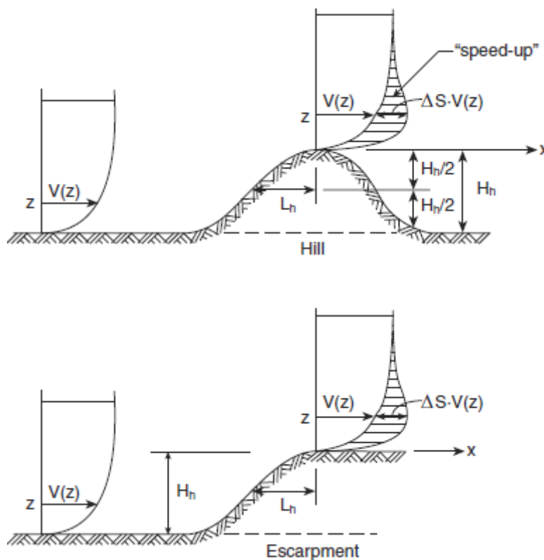
Figure 4.1.7.4. Speed-up of Mean Velocity on a Hill or Escarpment (1) Forming Part of Sentence 4.1.7.4.(2)
