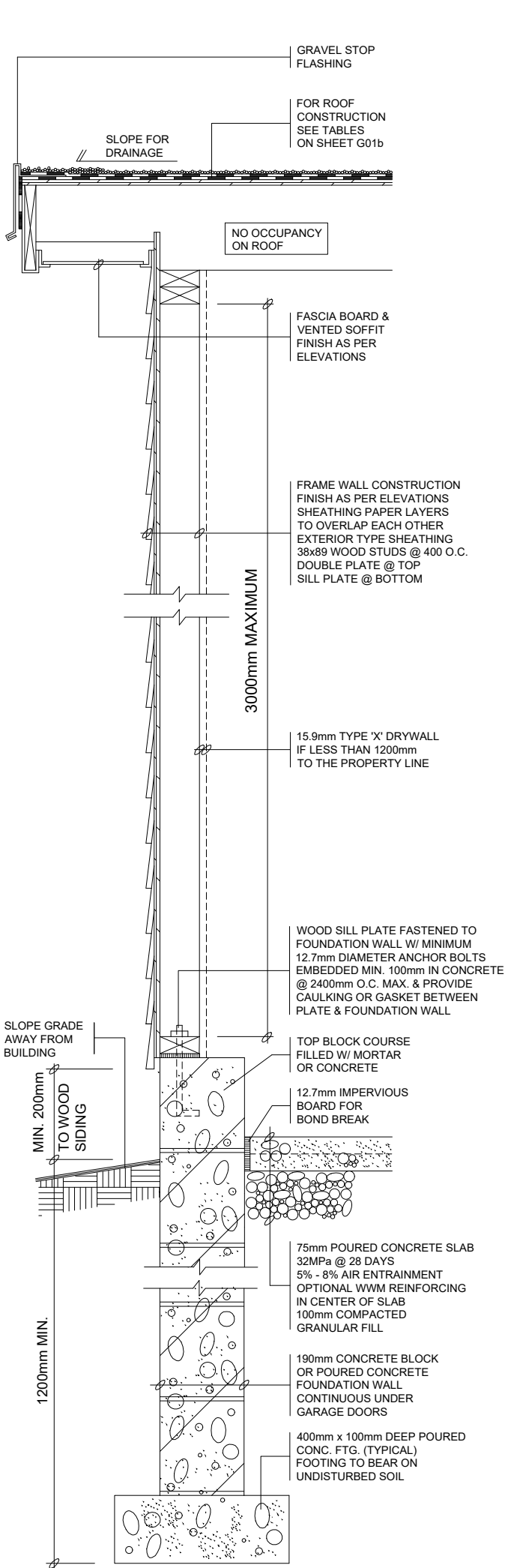
4 WALL SECTION
