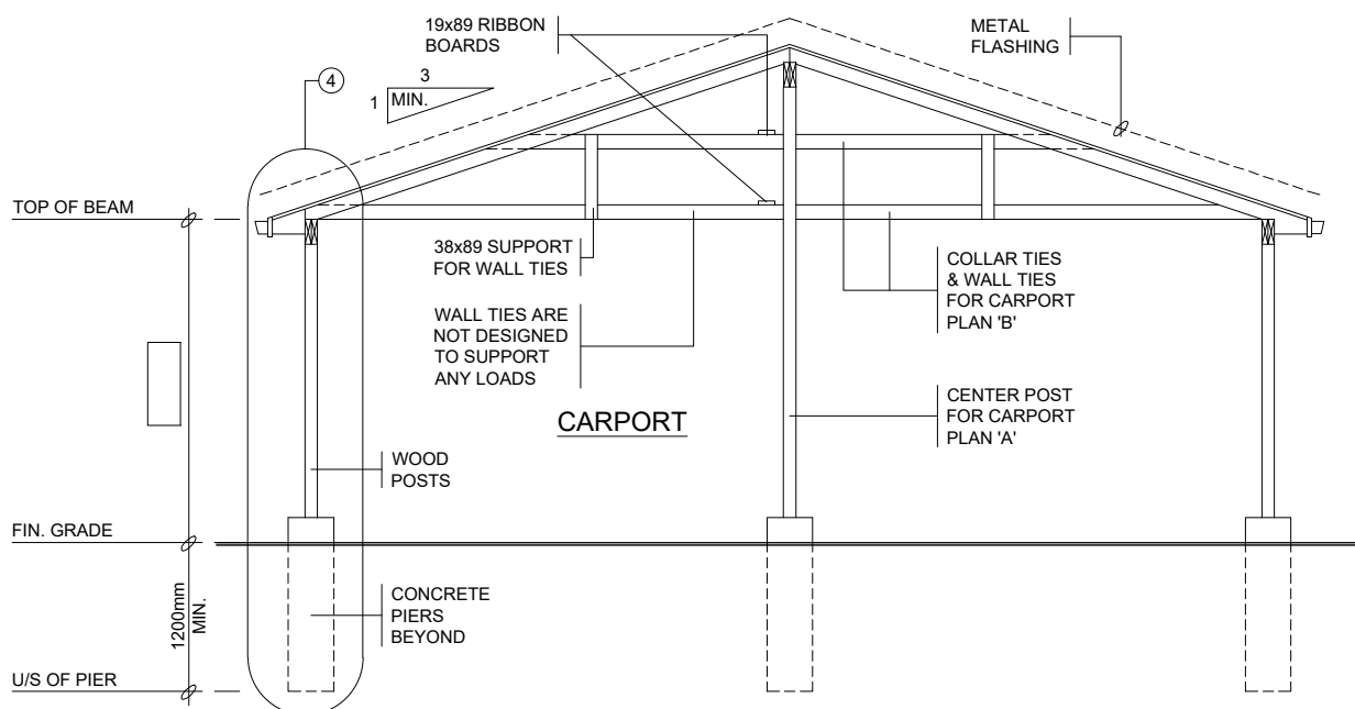
CARPORT SECTION
